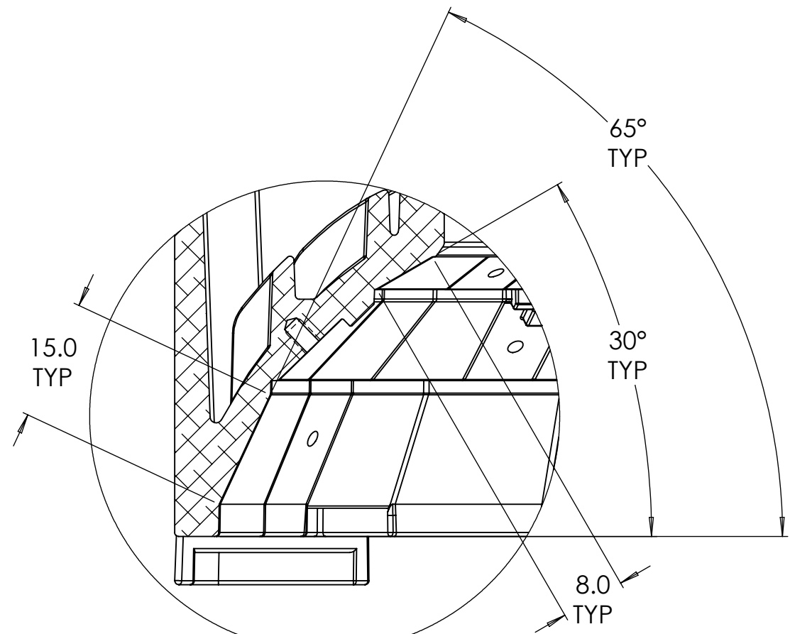
DETAIL C SCALE 3:2
